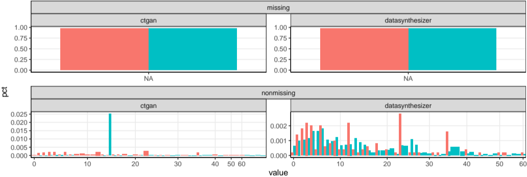
Figure 12: CTGAN does not correctly estimate the distribution, DataSynthesizer gets the median (10)
