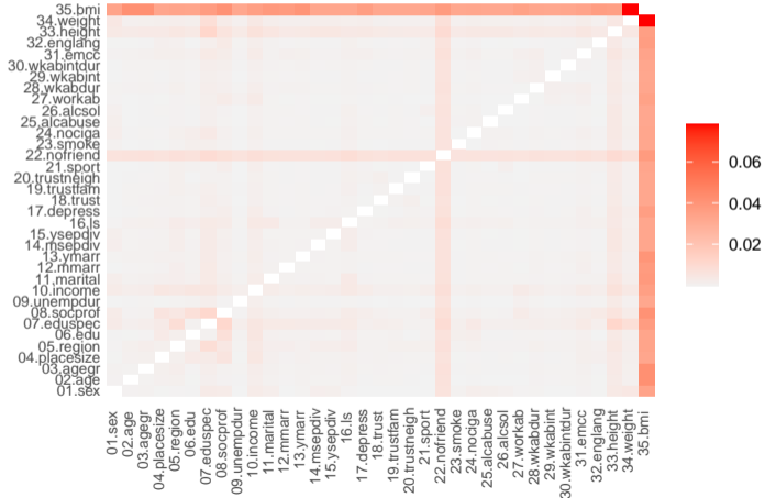
Figure 4: SD2011(b) – missing are numerical values < 0 and “ ” categorical values
