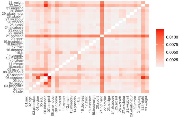
Figure 6: SD2011(c) – drop generated variables (bmi and agegr)
