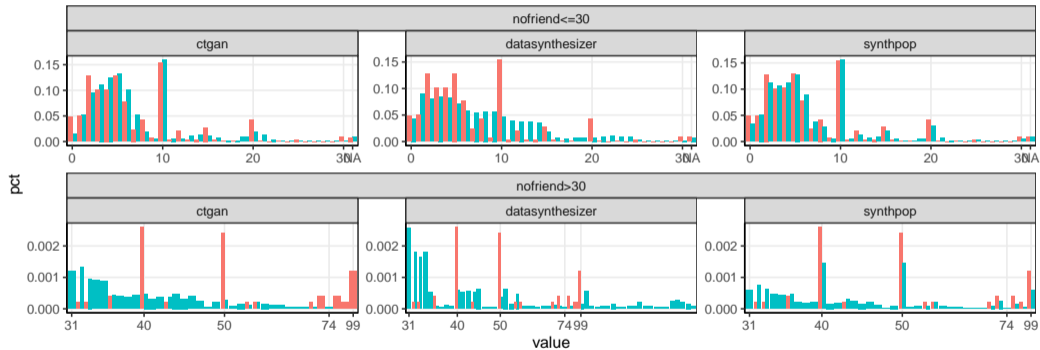
Figure 15: Synthpop captures the distribution
