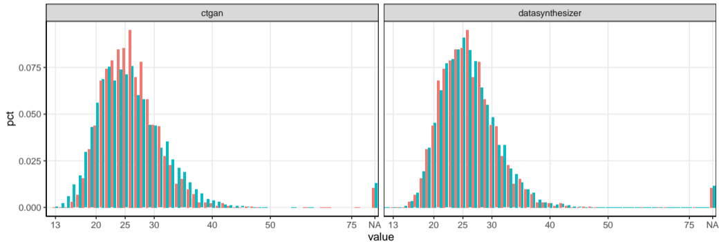
Figure 11: CTGAN/DataSynthesizer estimate the median, but CTGAN is skewed a bit more to the right
